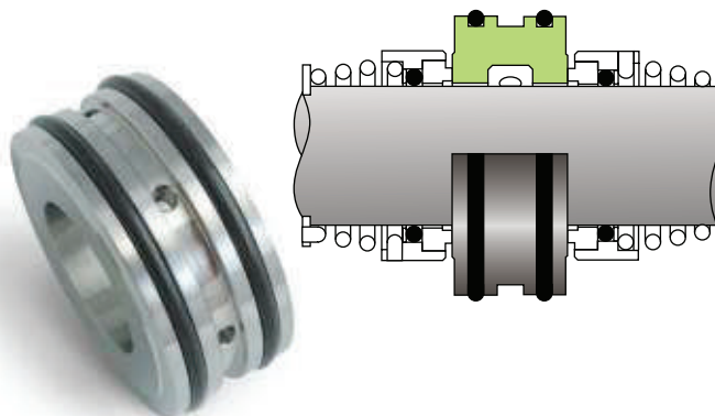
22mm Inboard encased rotary with Carbon Face
