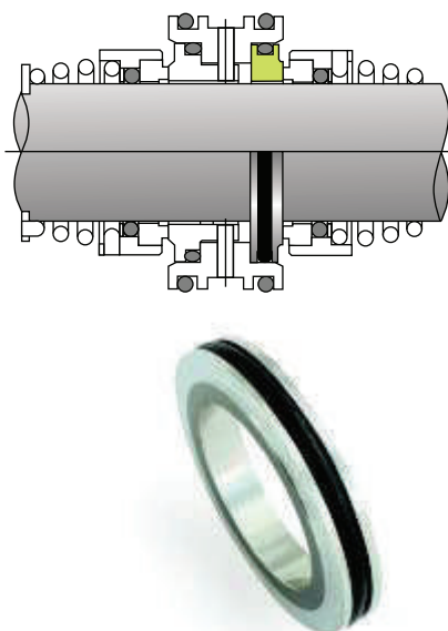
H type Insert with O ring
