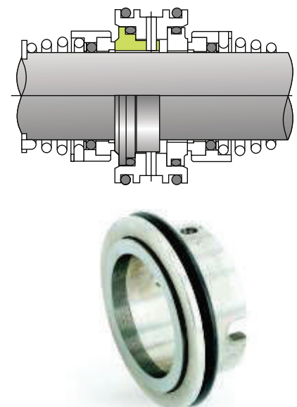
L type Insert with O ring
